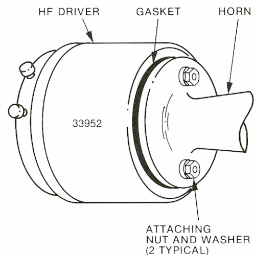
Figure 6. Horn/Driver Mounting
