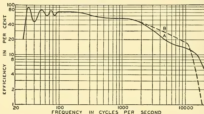
FIG. 8.16. Efficiency characteristic of a diaphragm coupled to the horn of Fig. 5.8 and driven by an aluminum voice coil of one-half the diaphragm mass in a field of 22,000 gauss. A . Without air chamber. B . With air chamber.
