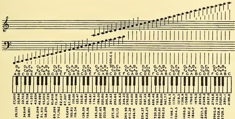
FIG. 13.14. The piano keyboard and the frequencies of the equally tempered scale as used in music according to the American Standard Pitch.
