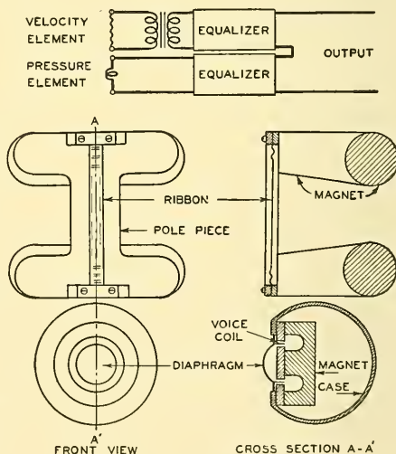
FIG. 9.25. Unidirectional microphone consisting of a ribbon type velocity element and a dynamic type pressure element.
