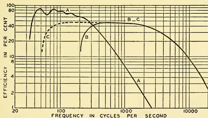
FIG. 8.15. A . Efficiency characteristic of a horn loud speaker employing the horn of Fig. 5.6 D with the dimensions multiplied by three and driven by 4 cones, 12 inches in diameter, with 5 gram copper voice coils operating in a field of 14,000 gauss. B . Efficiency characteristic of a horn loud speaker employing the horn of Fig. 5.5 D with the dimensions multiplied by one-half and driven by a diaphragm and an aluminum voice coil having a mass ratio of two to one operating in a field of 22,000 gauss. C . Same as B save that the horn dimensions of Fig. 5.5 D are multiplied by two.
