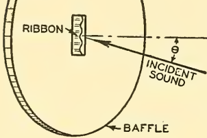
FIG. 9.17. A ribbon microphone with a large circular baffle.
