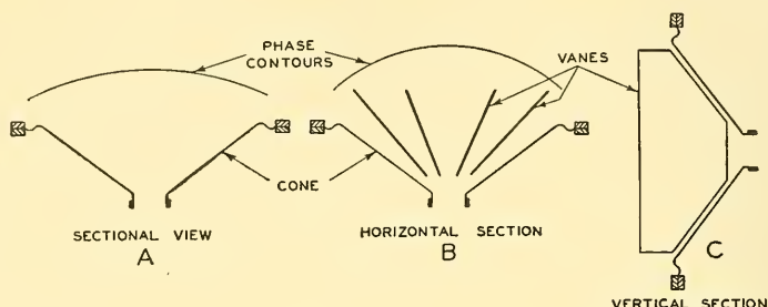
FIG. 7.20. High frequency sound distributors for direct radiator loud speakers. A. The contour of equal phase for a plain cone. B. The horizontal cross-sectional view of a cone with a vane distributor and the contour of equal phase. C. The vertical cross-sectional view of a cone with a vane distributor.
