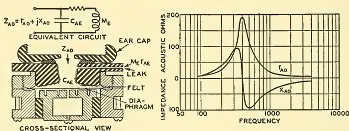
FIG. 11.15. A cross-sectional view of an artificial ear employing a standard condenser microphone and the equivalent electrical circuit of the acoustical system. The graph shows the resistive r_{A0} and reactive x_{A0} components of the acoustic impedance, looking into the aperture of the ear cap, as a function of the frequency. C_{AE} acoustic capacitance of the cavity. M_E and r_{AE} inductance and acoustic resistance of the leak.
