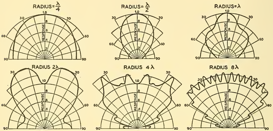
FIG. 2.6. Directional characteristics of a 120° arc as a function of the radius and the wavelength. The polar graph depicts the pressure, at a large fixed distance, as a function of the angle in the plane of the arc. The pressure for the angle 0° is arbitrarily chosen as unity.
