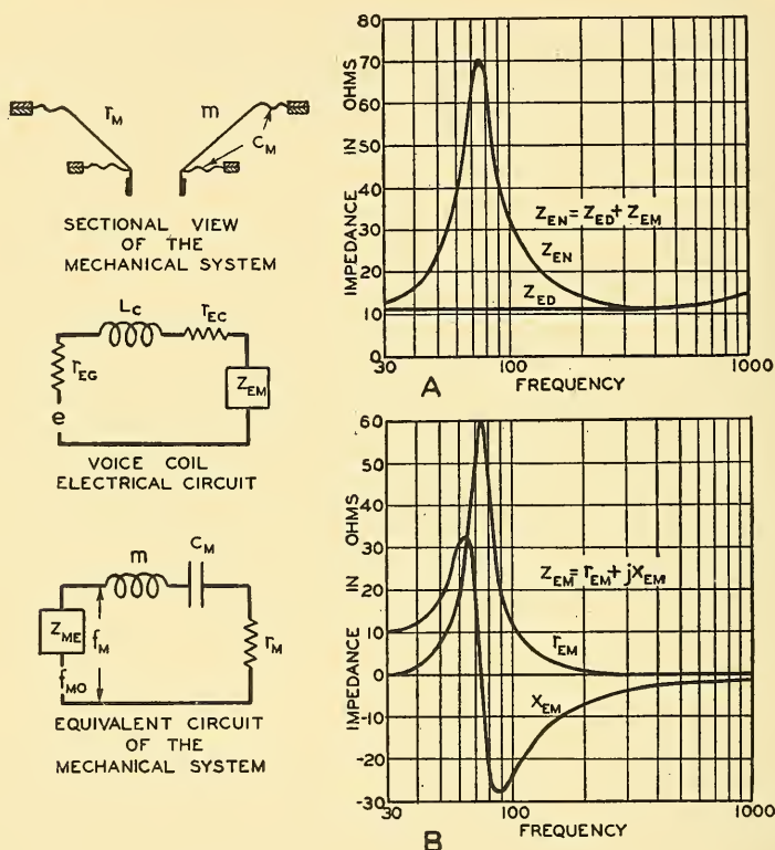
FIG. 7.3. Electrical and mechanical circuits of a dynamic loud speaker at the low frequencies.
