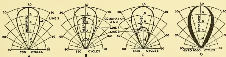
FIG. 9.40. A . The directional characteristic of line 3 at 700 cycles. B . The directional characteristics of lines 2 and 3 and the resultant at 950 cycles. C . The directional characteristics of lines 2 and 3 and the resultant of 1250 cycles. D . The directional characteristics of the microphone shown in Fig. 9.38 for the range from 85 to 8000 cycles fall within the shaded area.
