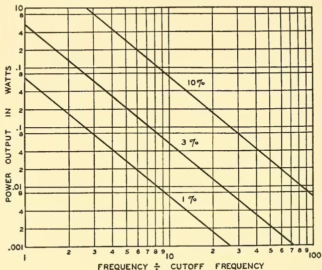
FIG. 8.8. The power output of infinite exponential horns, per square centimeter of throat area, for 1, 3 and 10 per cent distortion, as a function of the ratio of the frequency under consideration to the cutoff frequency.
