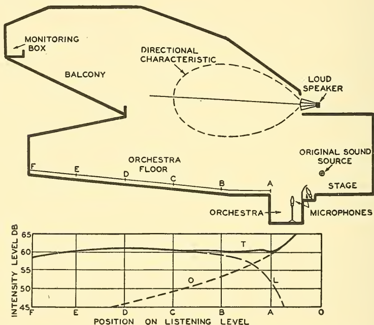
FIG. 12.4. Arrangement of the components of a sound re-enforcing system in a theatre. The graph shows the intensity level due to direct sound at the points indicated on the orchestra floor. Curve O, the intensity due to the original source of sound. Curve L the intensity level due to the loud speaker. Curve T the resultant intensity level.
