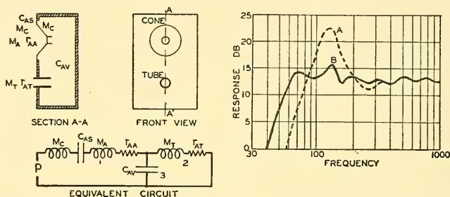
FIG. 7.11. Phase inverter loud speaker and the equivalent circuit of the acoustical system. M_C the inductance of the cone. C_{AS} the acoustic capacitance of the suspension system. M_A and r_{AA} the inductance and the resistance of the air load upon the front of the cone. C_{AV} the acoustic capacitance of the cabinet volume. M_T and r_{AT} the inductance and acoustic radiation resistance of the tube. The pressure p of the generator in the acoustic system is the force generated in the voice coil divided by the area of the cone. The pressure response frequency characteristic of the phase inverter loud speaker is labeled B on the graph. The pressure response frequency characteristic of a loud speaker in a typical cabinet having the same volume as the phase inverter is labeled A on the graph. (After Dickey, Caulton and Perry.) (Courtesy of The Blakiston Company from Olson and Massa, "Applied Acoustics.")
