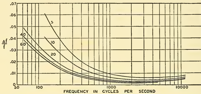
FIG. 13.12. The variation of \Delta f/f with frequency for various sensation levels. \Delta f is the change in frequency. Sensation level is level above threshold. (After Shower and Beddolph.)
