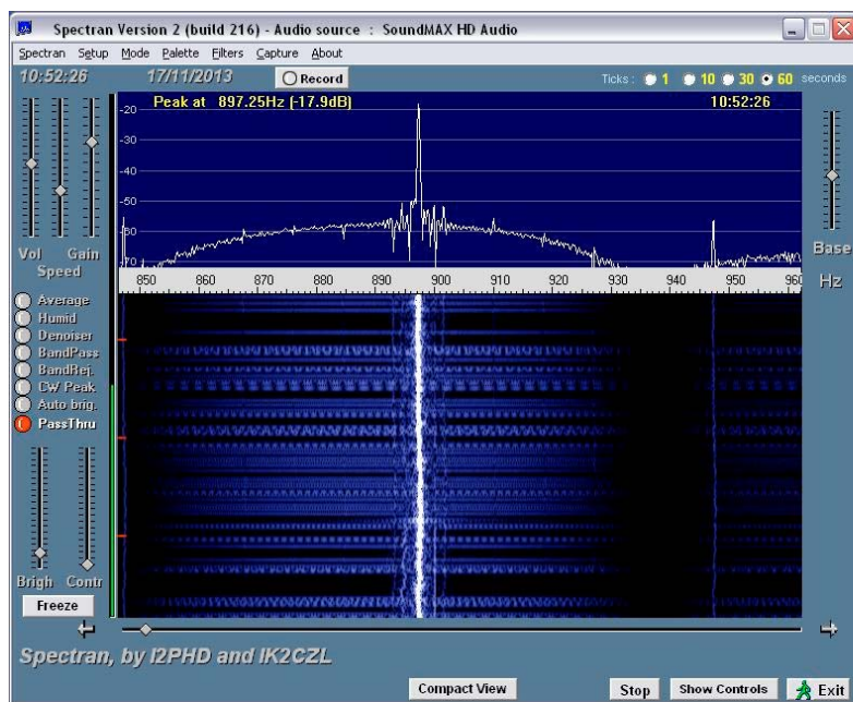
Figure 9 VE2ZAZ GPS Disciplined Oscillator showing excellent short term frequency stability, but with a fixed offset error that 'will' eventually be corrected – very slowly, perhaps, by the frequency-counter-based correction loop.
