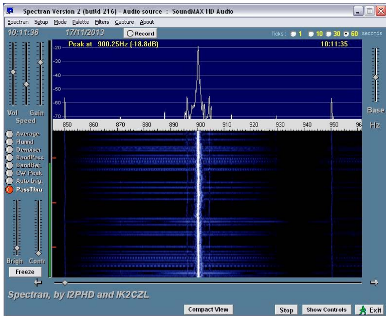
Figure 3 LPFRS01 Rb Source, 9 minutes after Turn On
