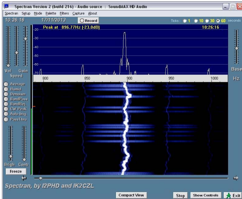
Figure 8 Cheap and Simple GPSDO, expanded scale
