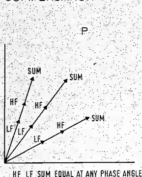
FIG. 1b KINOSHITA PHASE COMPENSATION
