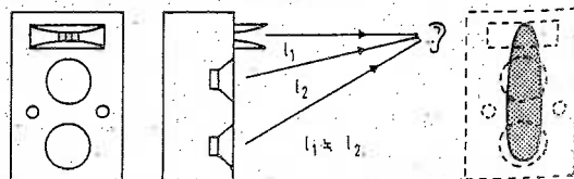
FIG. 4 CONVENTIONAL VERTICALLY ARRANGED DOUBLE WOOFER SYSTEM
