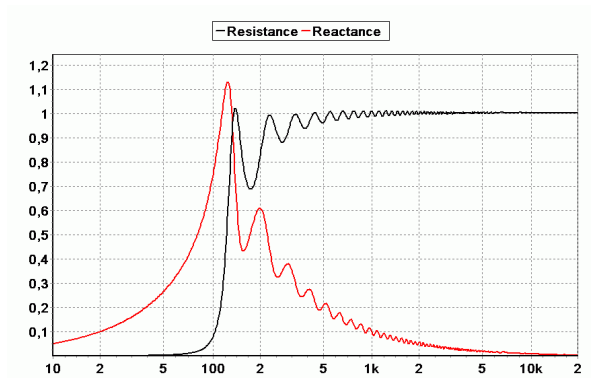
Figure 23: Throat impedance of a spherical wave horn.
