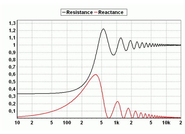
Figure 7: Finite exponential horn terminated by an infinite pipe.
