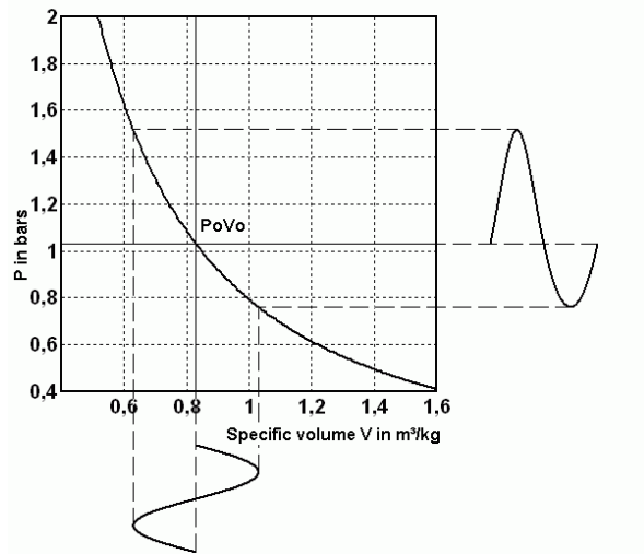
Figure 40: Adiabatic curve for air.
