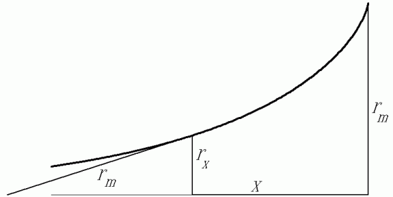
Figure 17: Dimensions of the tractrix horn
