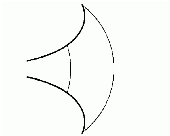
Figure 22: Spherical wave horn folding back.
