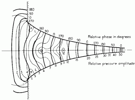
Figure 15: Wave-fronts in an exponential horn at 800 Hz. [4]
