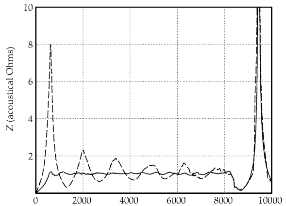
Figure 1: Throat impedance of a typical constant directivity horn (- - -) and a tractrix horn (—). [1]
